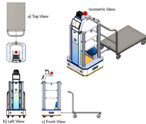
Figure 4. design of paramedic assistant robot 2.0
