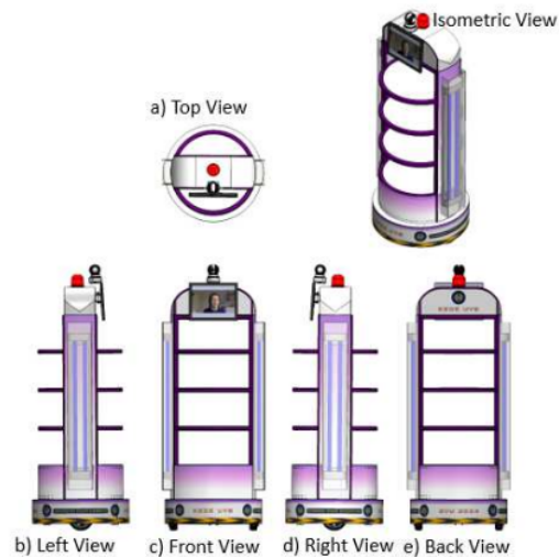
Figure 3. design of paramedic assistant robot 1.0
